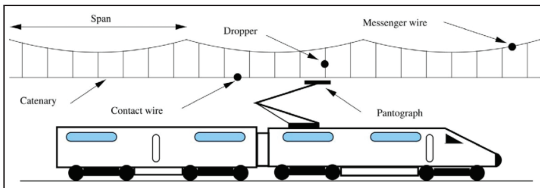
Figure 1: A sample train with pantograph and overhead catenary system (Lopez-Garcia et al., 2006).
