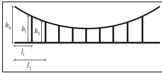
Figure 2: Contact wire cross-section
