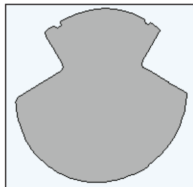
Figure 2: Contact wire cross-section
